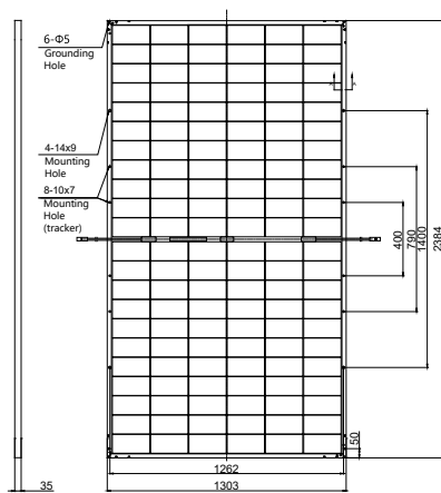
Rear View
